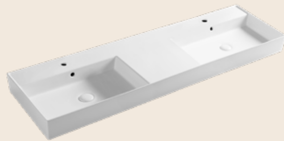
Art. DRP4316DB101 DROP 160 doppia vasca / double bowl cm 160x46x15 h
